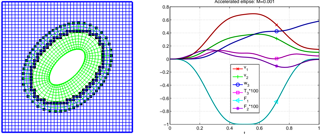
Figure 10: Accelerated ellipse. Left: overlapping grid \mathcal{G}_{\text{re}}^{(1)} at time t = 0 . Right: time histories of the rigid body velocity (v_1, v_2) , angular momentum w_3 , torque T_3 and forces (F_1, F_2) for an ellipse of mass m_b = 10^{-3} and moment of inertia I_3 = 10^{-3} using the old algorithm (black lines) and new algorithm (using grid \mathcal{G}_{\text{re}}^{(2)} ). ( T_3 and F_2 are scaled by a factor of 100 for graphical purposes). The force shown on the body does not include the contribution from the external body force.
